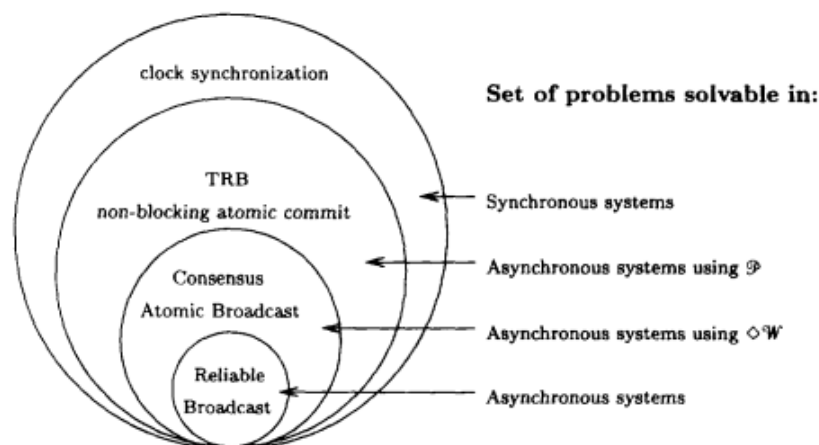
FIG. 9. Problem solvability in different distributed computing models.
